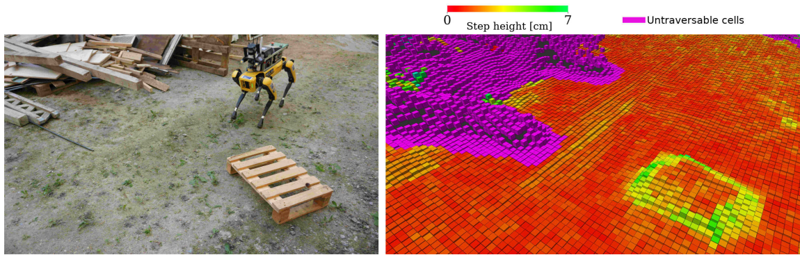
Figure 9. (Left) Outdoor area with rough and untraversable terrains. (Right) Terrain model built from LiDAR mounted on a quadruped robot with a visualized step height \Delta(v) .
