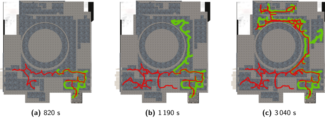
Figure 17. Visualization of the exploration progress by colored paths of the exploring ground robots at particular time instances of Environment 5 (Figure 16e). After 820 s, the robot with the green path separates from the other robot at the main crossroad since waypoints near the path marked by the red color had higher ranks than the waypoint located at the not yet visited part of the environment. After 1190 s, the robot with the red path returns to the main crossroad. Since the area shown in the lower part of the visualized environment map is explored, the robot enters the second part of the environment already being explored by the other robot. After 3040 s from the mission start, the environment is explored by the robots with partially overlapping paths. Such behavior is intentional, and it increases the system’s robustness.
