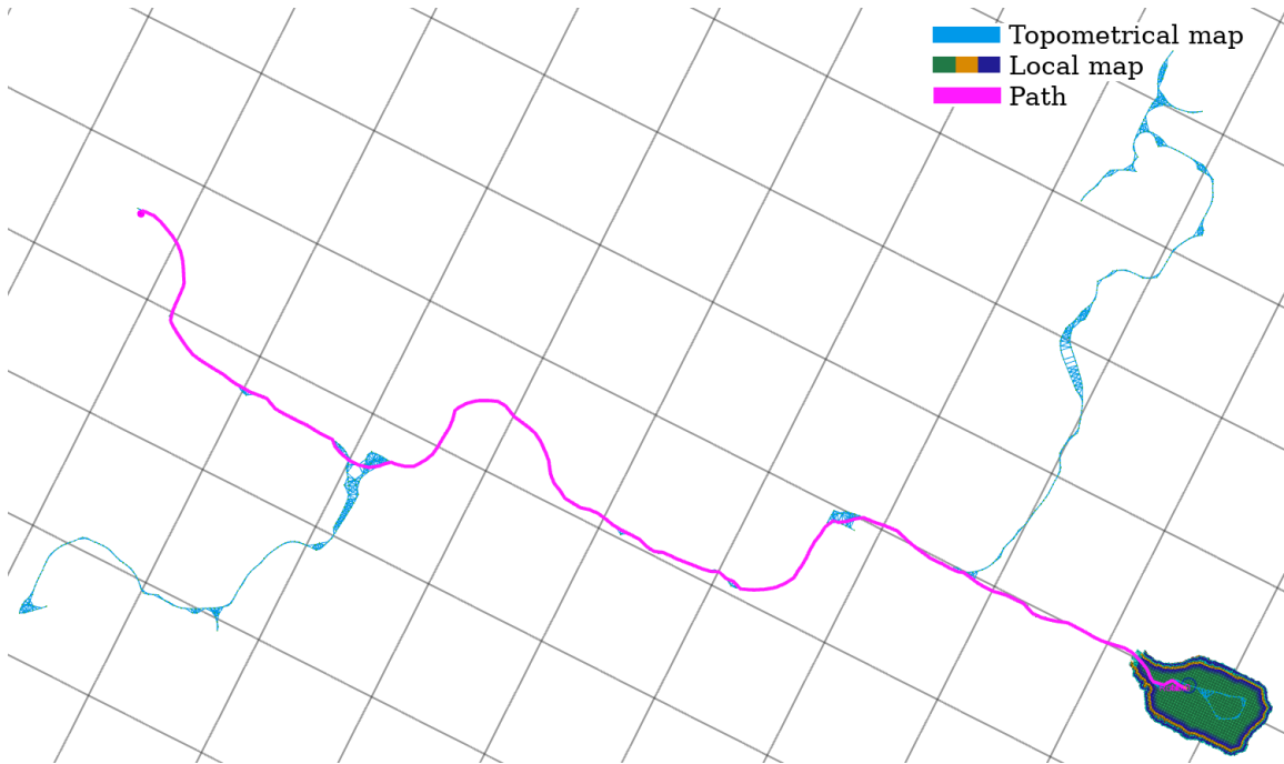
Figure 14. Topometrical map with highlighted path and a local map used for benchmarking the path planning using the Intel 8th generation of the i7-class CPU with 32 GB RAM. The cell size of the visualization grid is 20 m.
