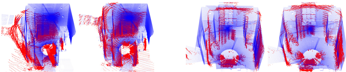
Figure 5. The left and right images show unaligned and aligned clouds in marker frame identification using a dense scan of a small room. The robot cloud (red) is aligned with the reference cloud (blue). Notice the density and precision of the reference (blue) cloud obtained by the Leica BLK-360 laser scanner.
