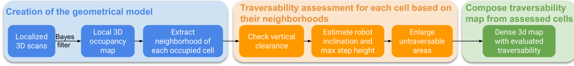
Figure 6. A schema of the local elevation map creation and traversability assessment.
